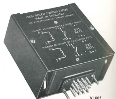
Solid-state high speed switch, Type F 3070
