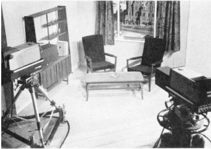
LEFT: A section of the Marconi stand at the British Industrial Exhibition, Moscow, showing Broadcasting Division's television studio. There were two Mark V cameras working here
