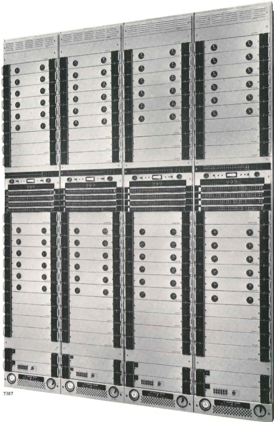
Channelling equipment manufactured by Automatic Telephone & Electric Company Limited, as supplied to New Zealand. This equipment carries 96 channels and is used with Multi-Channel Radio Equipment.
